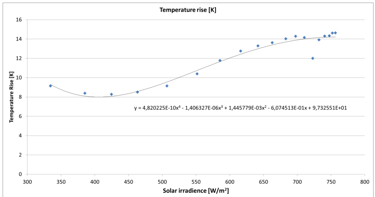
Figure 2 - Temperature rise
