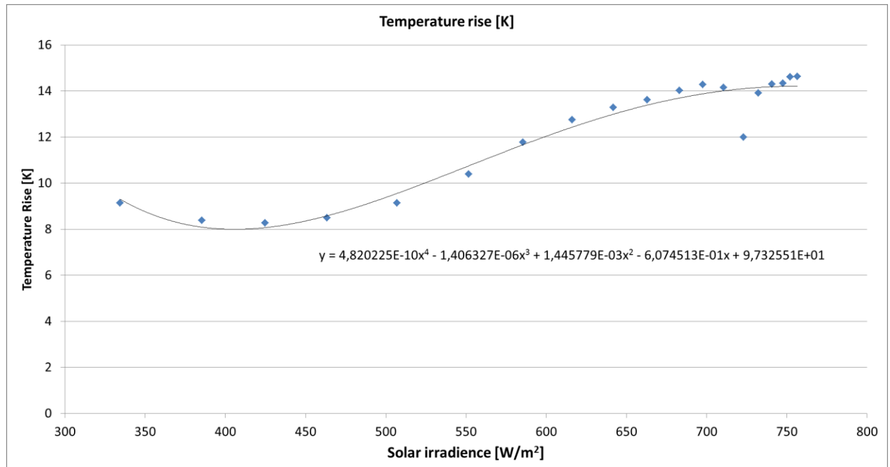
Figure 3 - Temperature rise
